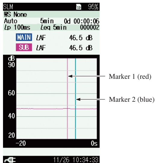
Time-Level screen
